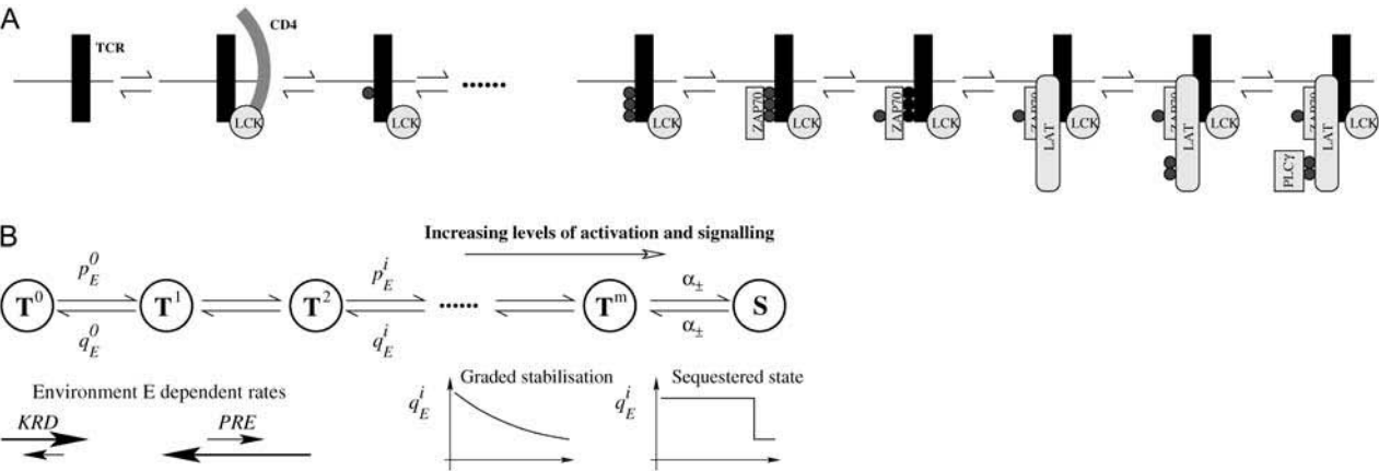
FIGURE 2 (A) Schematic for the activation step sequence of events leading to a signaling competent signalosome (● represents tyrosine phosphorylation). (B) Mathematical model of activation sequence with trends shown for the event rates in the different environments, (left inset), and two models for stabilization of the signalosome through reduced dephosphorylation at high levels of activation (right inset). Index i labels the activation step and E denotes the environment (either KRD or PRE).
