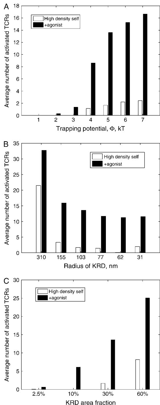
FIGURE 8 Average number of activated TCRs over the first 2000 s under variation of (A) trapping potential \Phi , (B) KRD radius (area fraction of KRDs remains 30%), and (C) KRD area fraction f . The number of KRDs in B are 1, 4, 9, 16, 25, and 100, respectively. The two cases are high-density self (open bars) and high-density self plus agonist (solid bars). Unvaried parameters as in Table 1.
